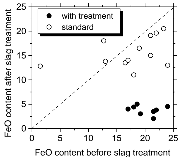
Fig.11 Reduction of FeO content in ladle slag by ladle slag reduction treatment [58]
